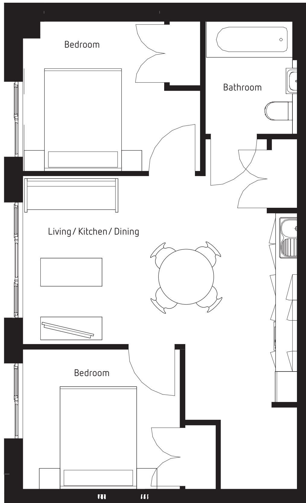
2-Bedroom Apartment Type 02B 7 units 550 sq.ft
