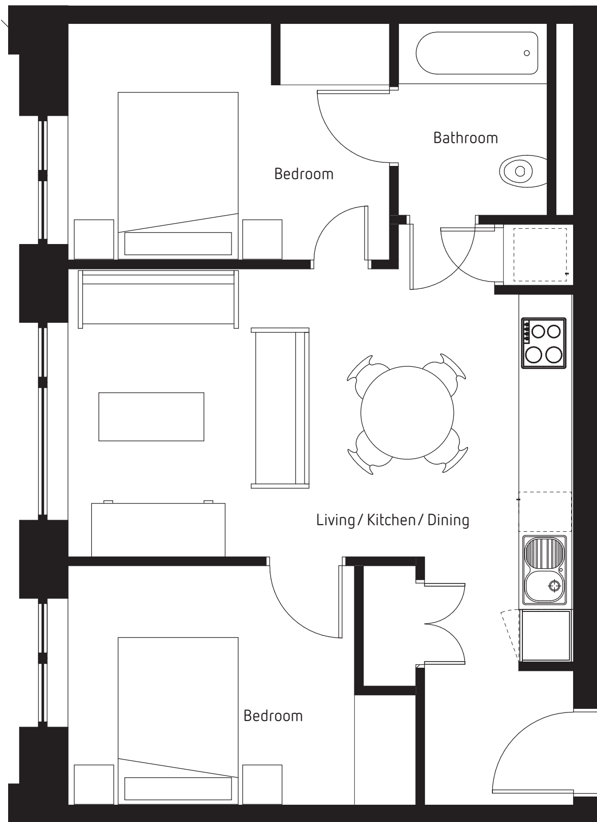
2-Bedroom Apartment Type 02 7 units 536 sq.ft
